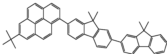
compound A3
