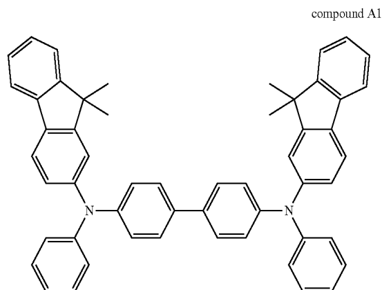
compound A1
